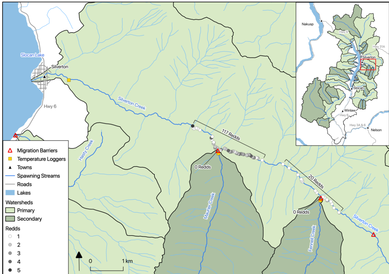
Figure 2. Bull Trout barriers and redd assessment results for Silverton Creek and tributaries, 2018.
